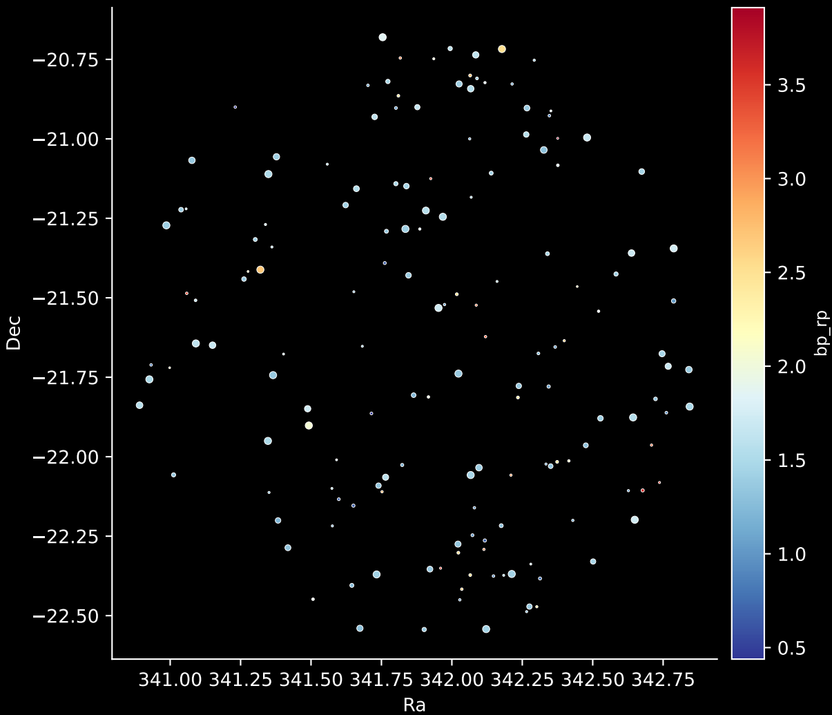
APOGEE DR17 Field: [352+22-O] Stars: 157
