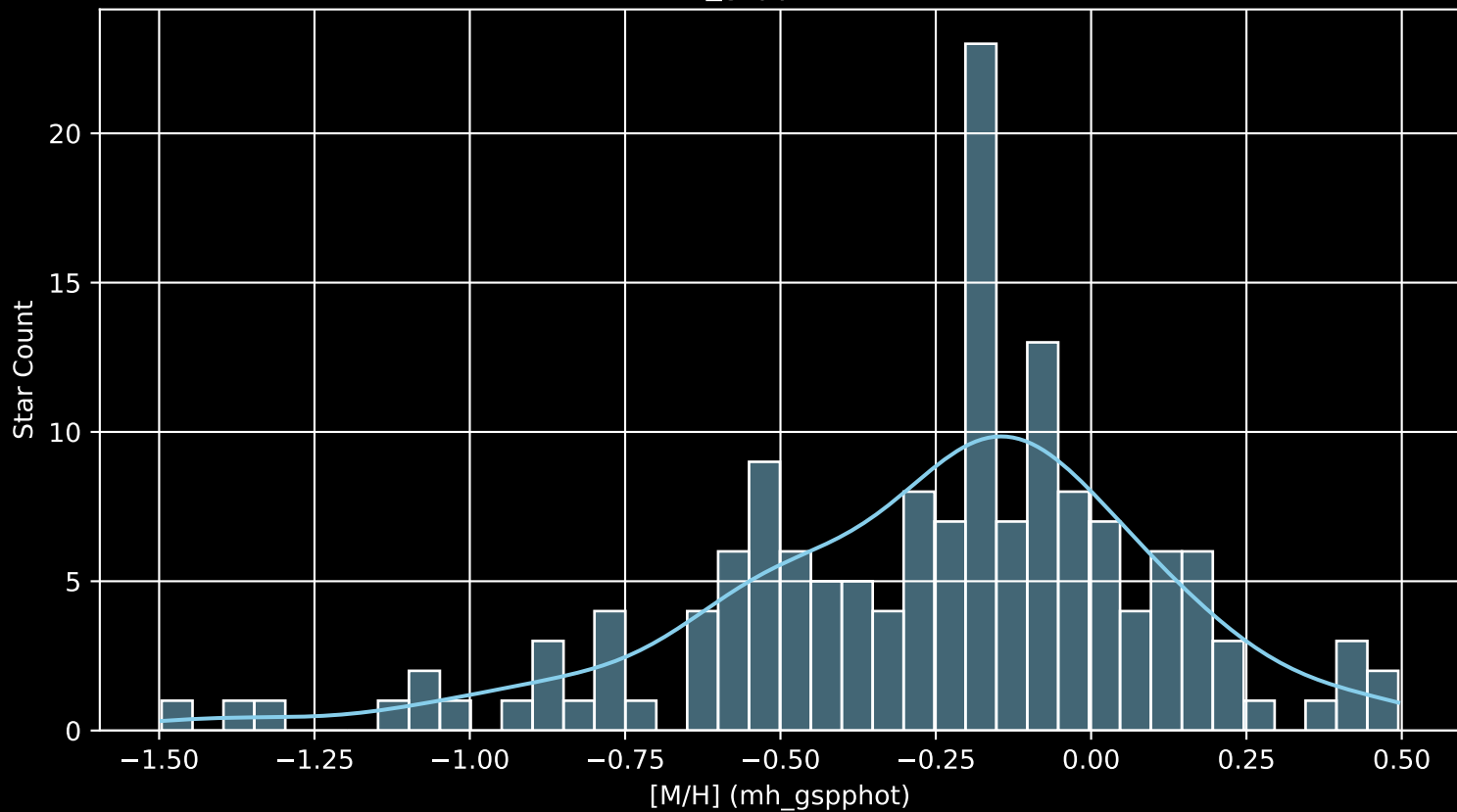
APOGEE DR17 Field: [352+22-O [M/H] (mh_gspphot) (n= 155)
