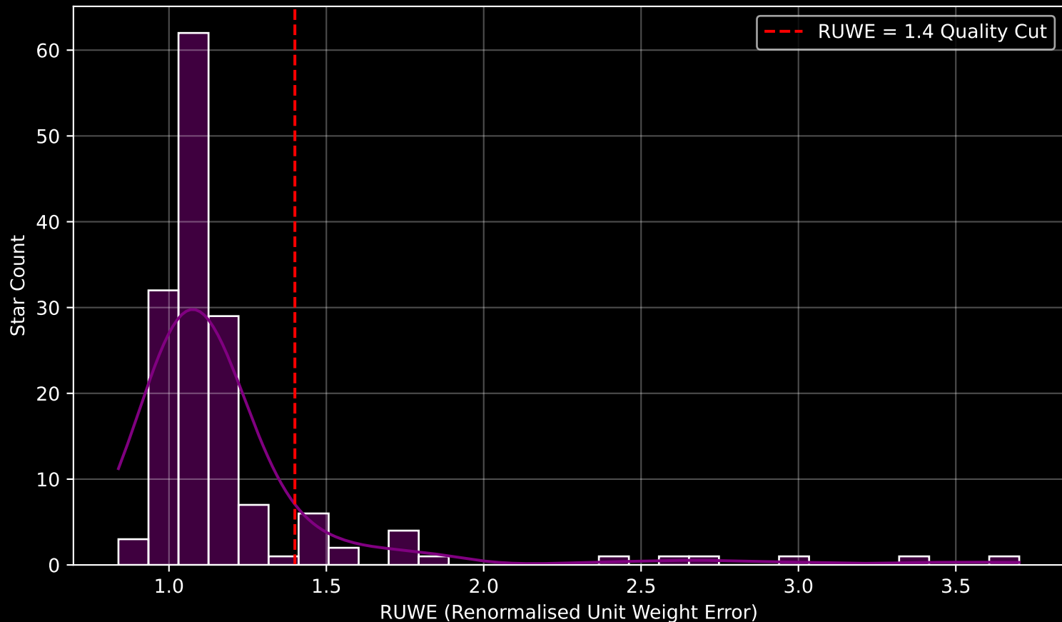
GAPOGEE DR17 Field [352+22-O] RUWE Distribution (n= 153)
