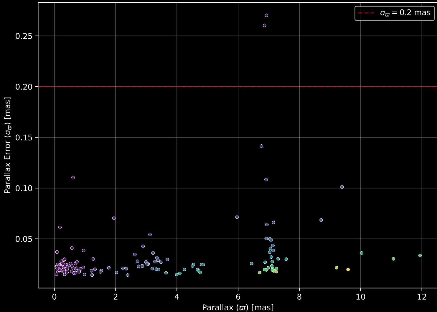
APOGEE DR17 Field: [352+22-O] Parallax Quality (n= 157)
