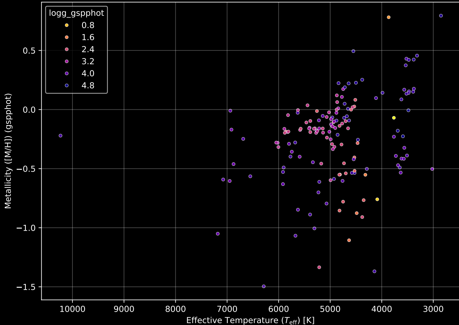
APOGEE DR17 Field: [352+22-O] Stellar Population Parameters (n= 157)
