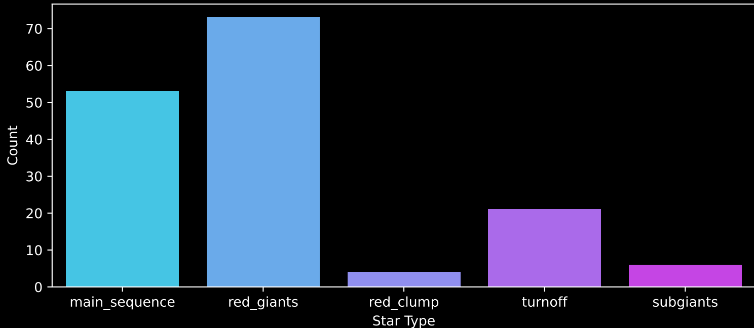
APOGEE DR17 Field: [352+22-O] Count plot of Star Type
