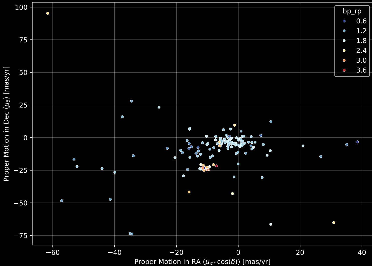
APOGEE DR17 Field: [352+22-O] Proper Motion Diagram (n= 157)
